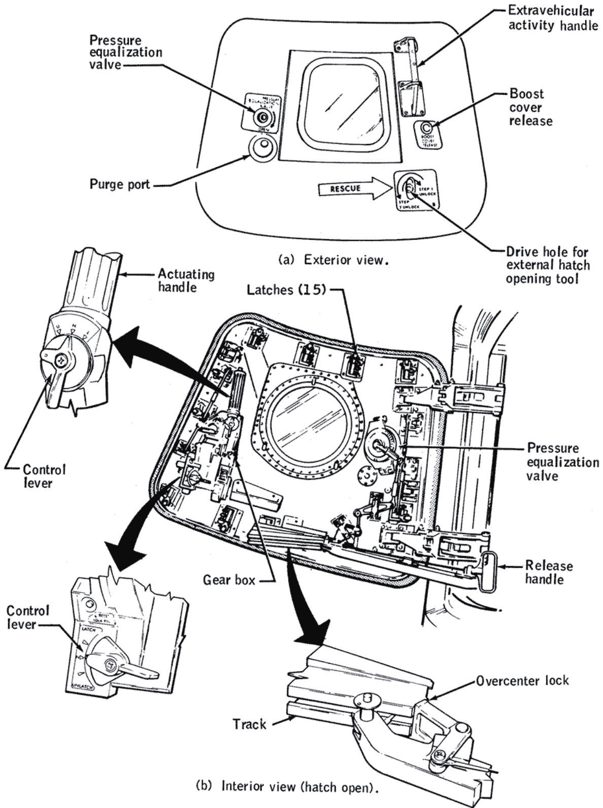
Figure 4-11.- Block II side hatch configuration.
