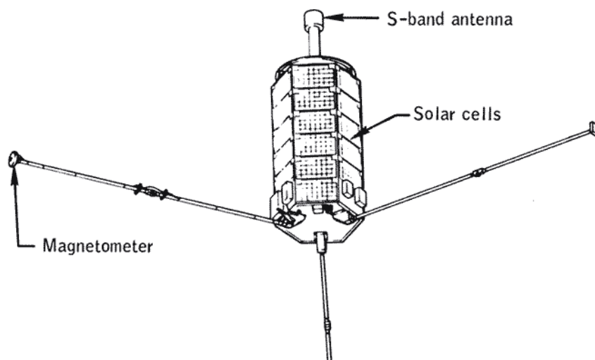
(b) Deployed subsattellite
