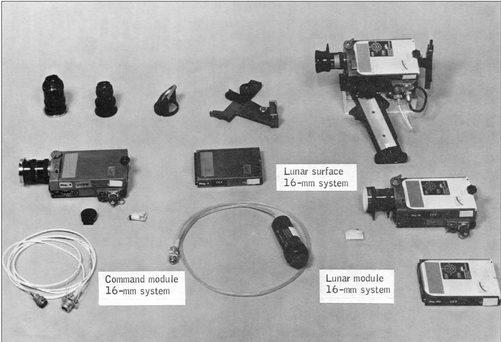
Figure 6-4.- The 16-mm sequence camera system.
