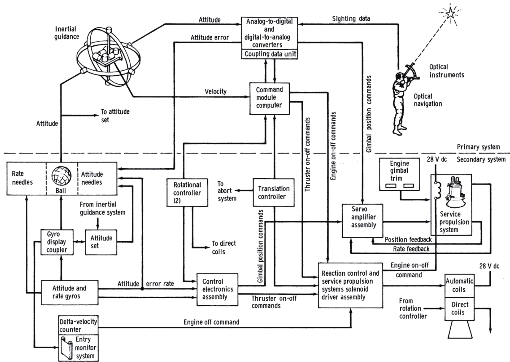
Figure 4-17. - Block II Command and service module guidance, navigation, and control system.
