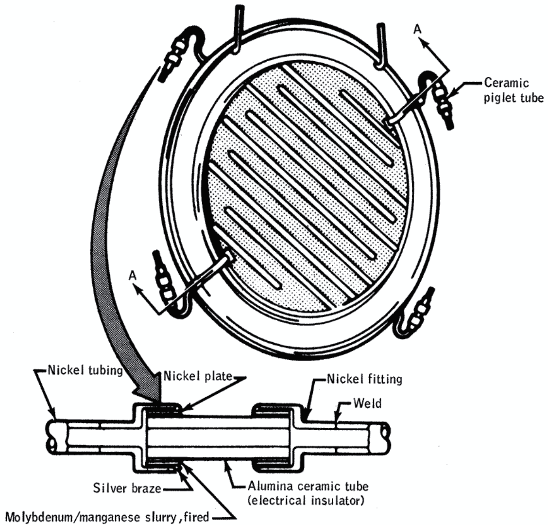
Figure 4-16.- Single-cell assembly.
