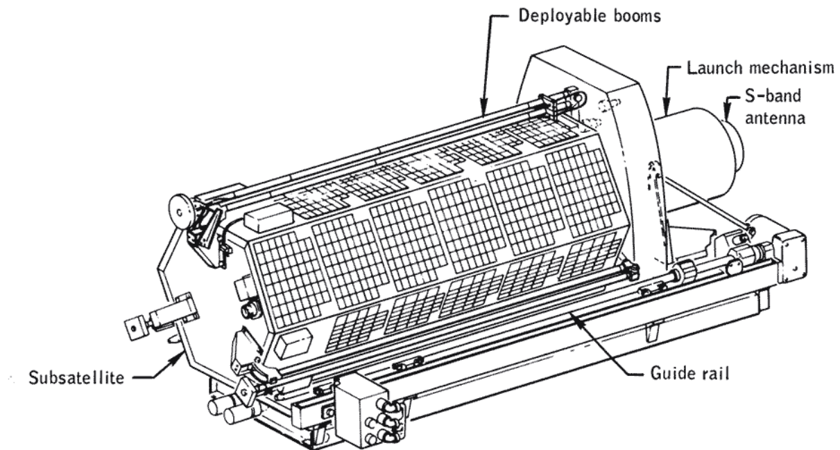
(a) Subsattellite predeployment configuration
