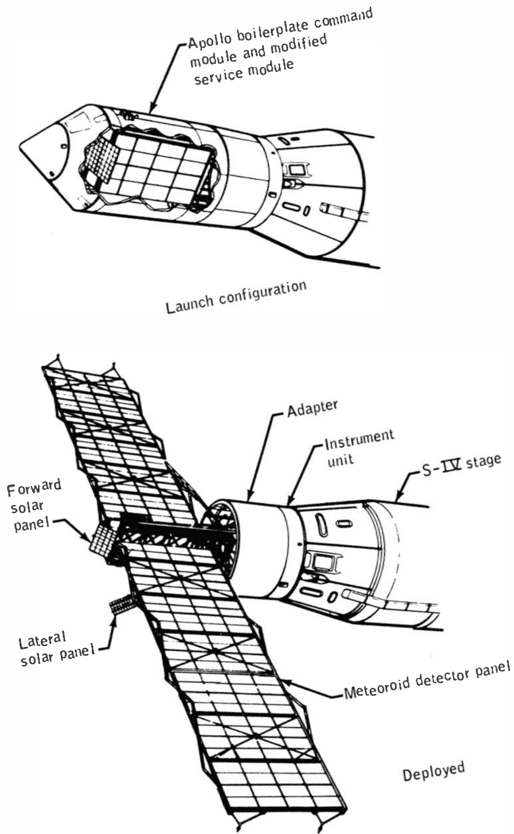
Figure 2-3.- Deployment of Pegasus satellite.
