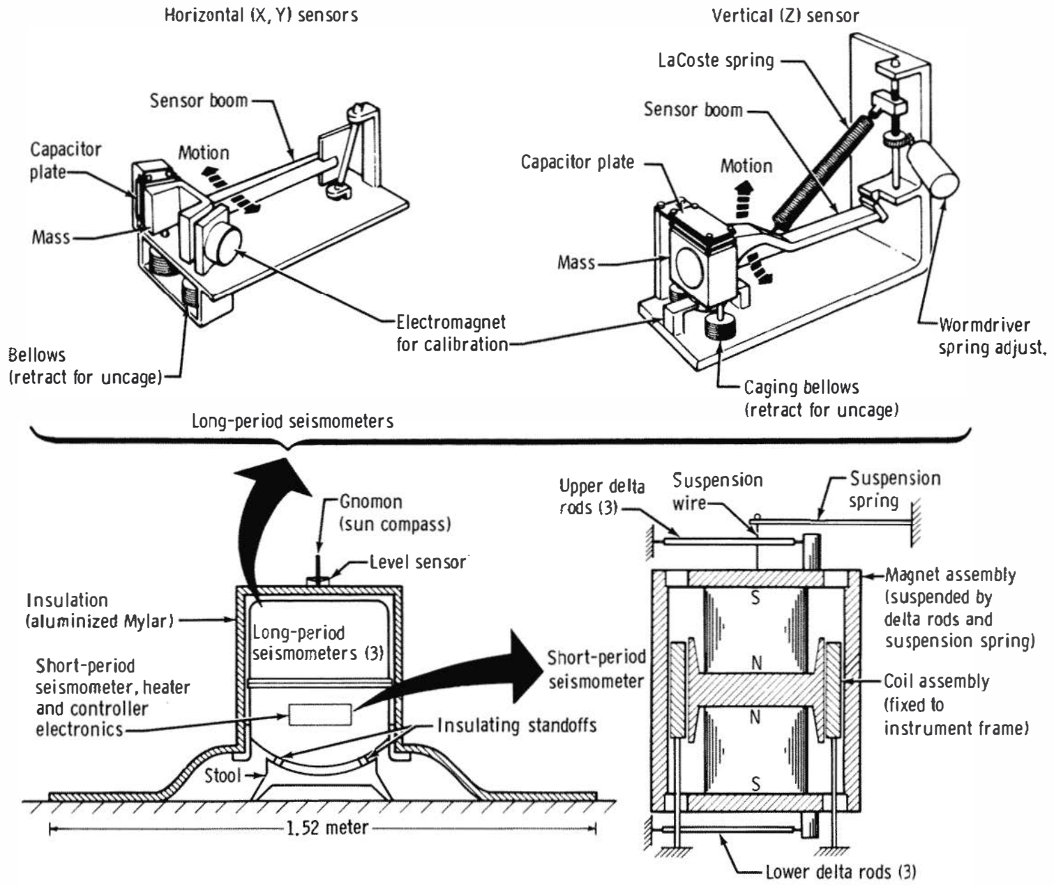
Figure 3-21. - Seismometer elements.
