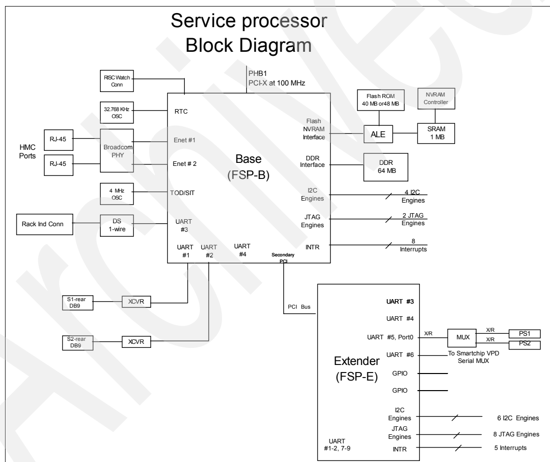
Figure 2-12 Service processor block diagram
