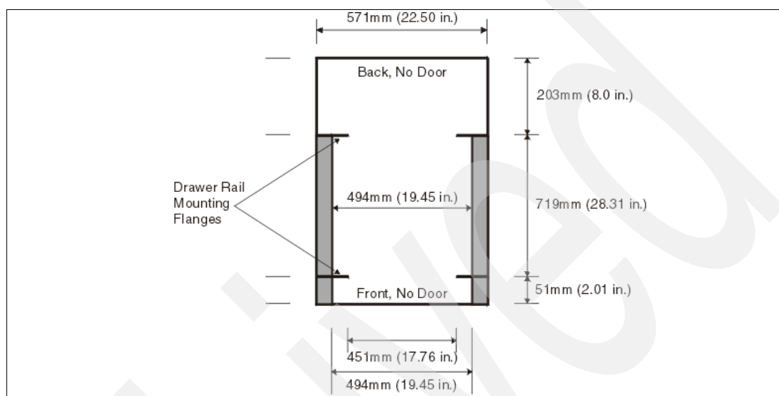
Figure 1-4 Top view non-IBM rack specification dimensions
