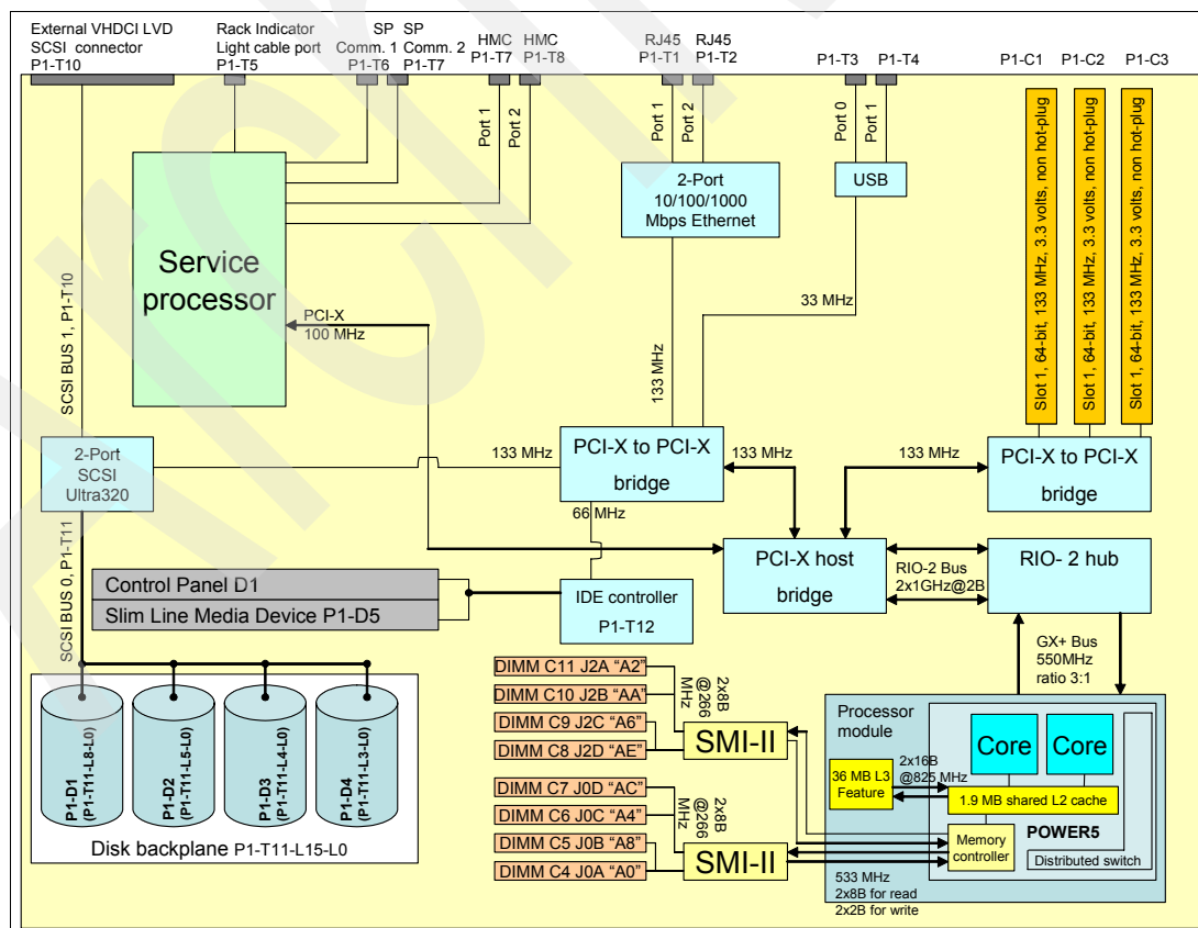
Figure 2-1 p5-510 server logic data flow
