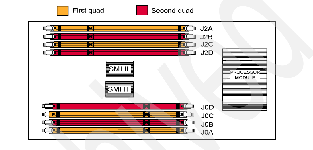
Figure 2-4 Memory placement for the p5-510 server
