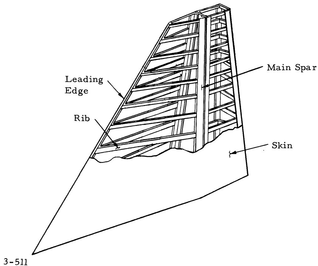
Figure 21-7. Fin, S-IC
