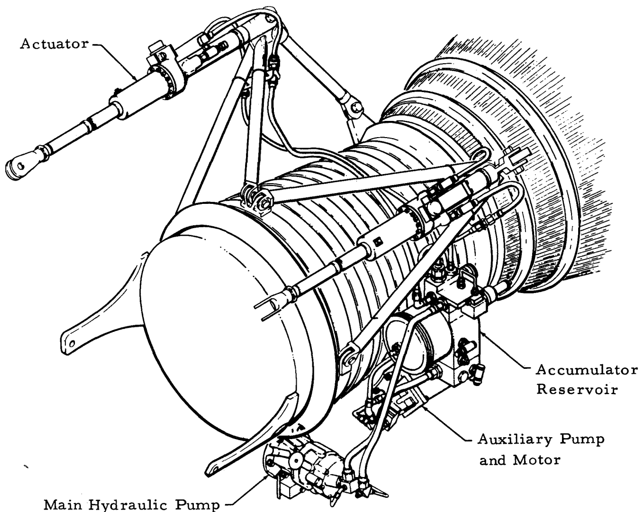
Figure 9-5. Engine Gimballing System Components
