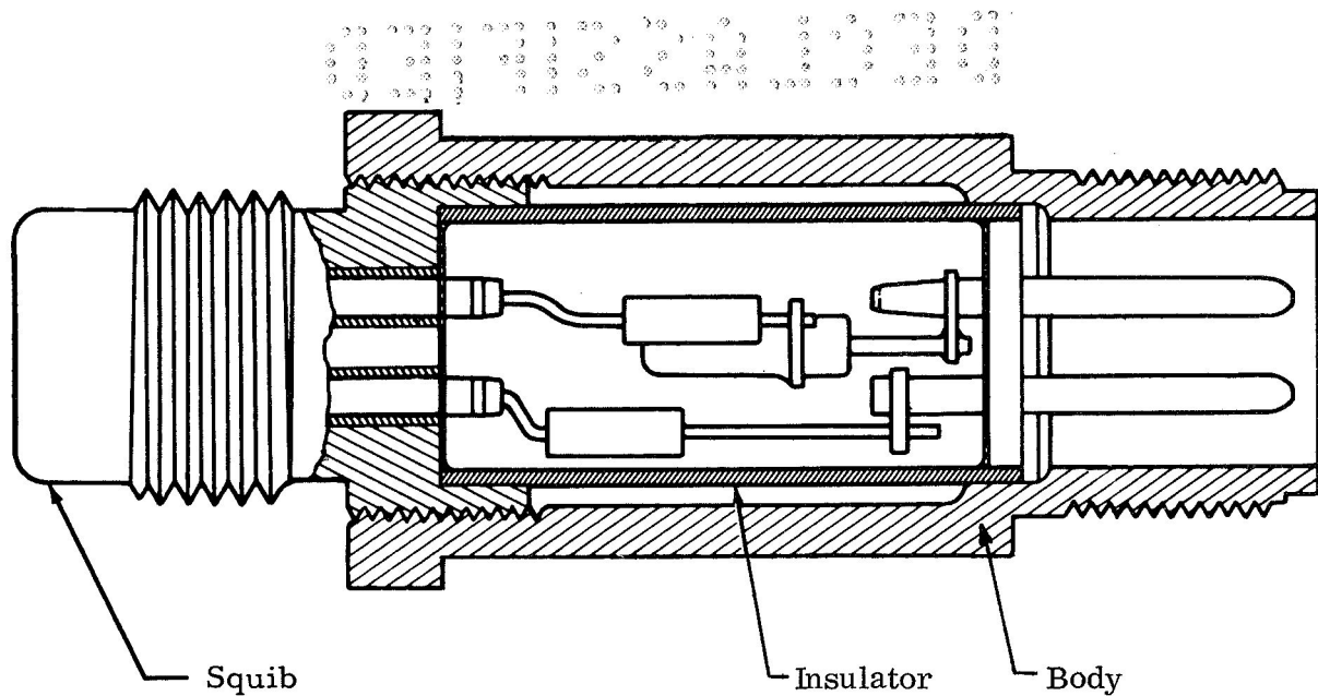
Figure 9-11. Solid-Propellant Gas Generator Initiator
