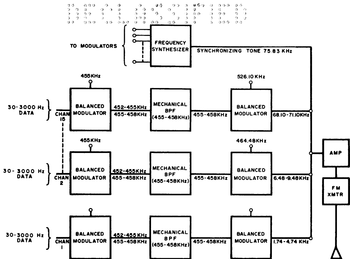
Figure 20-10. SS/FM Telemetry System, Saturn V
