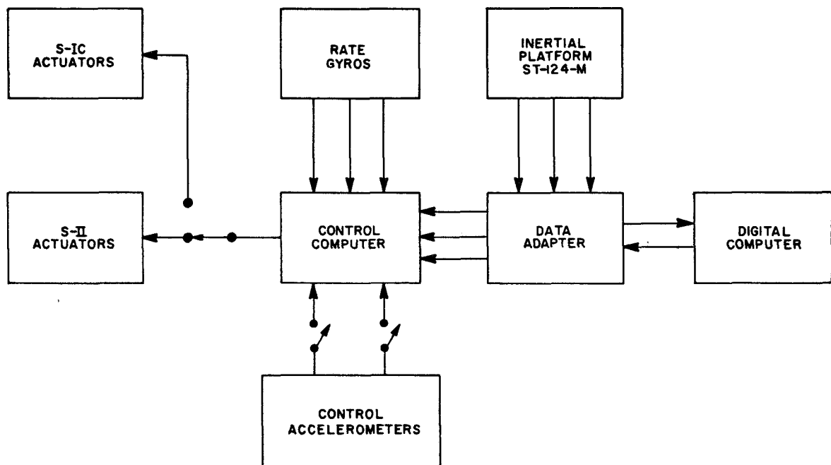
Figure 20-15. Thrust Vector Control System for S-IC and S-II Stages
