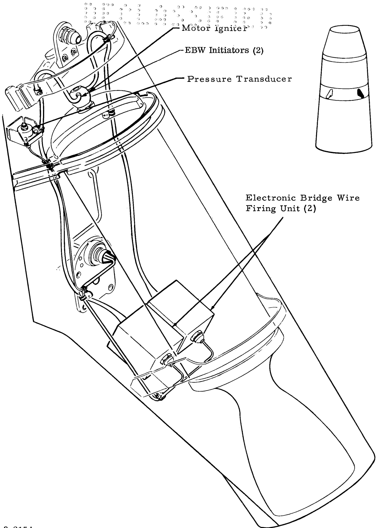
Figure 9-20. Ullage Motor Ignition System, S-IV
