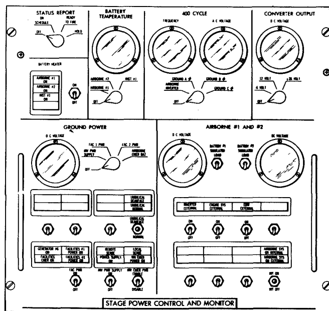
Stage Power Control and Monitor Panel
