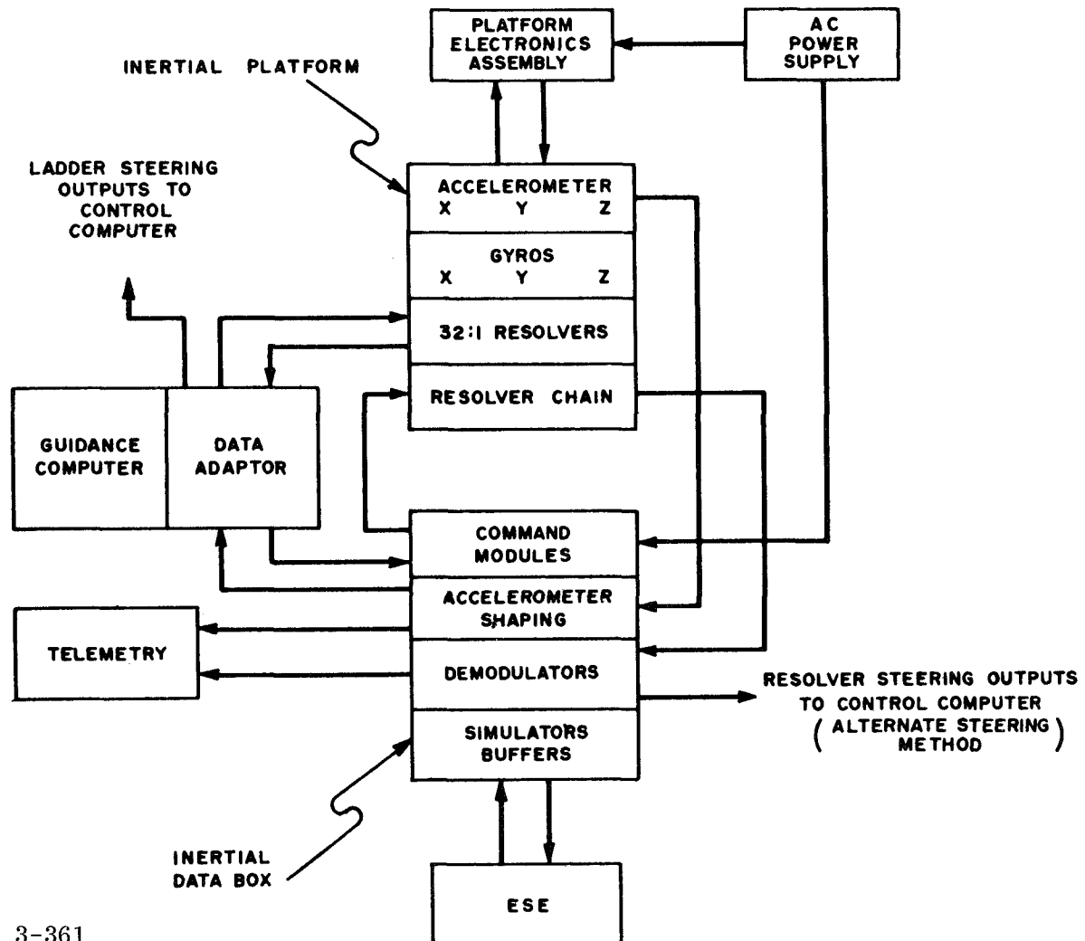
Figure 20-33. Guidance System Interconnection Block Diagram
