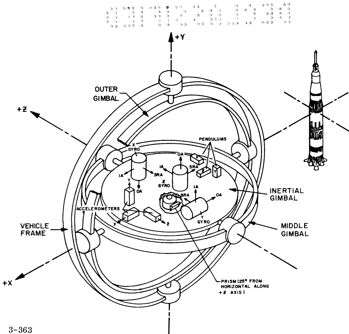
Figure 20-35. ST-124 M Gimbal Configuration
