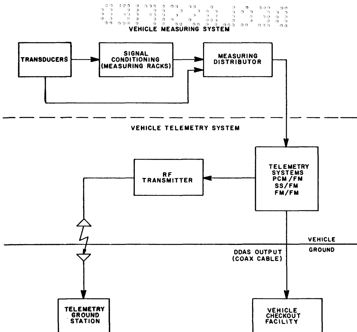
Figure 20-5. Instrumentation System, Saturn V
