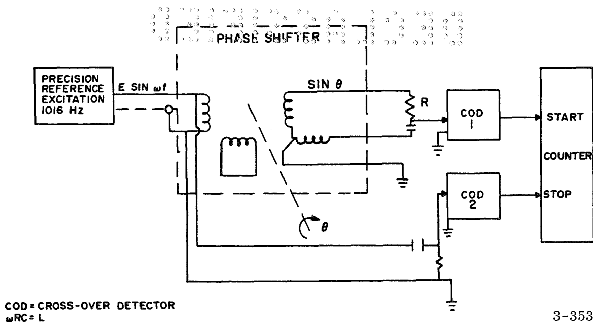
Figure 20-25. Angle Digitizer
