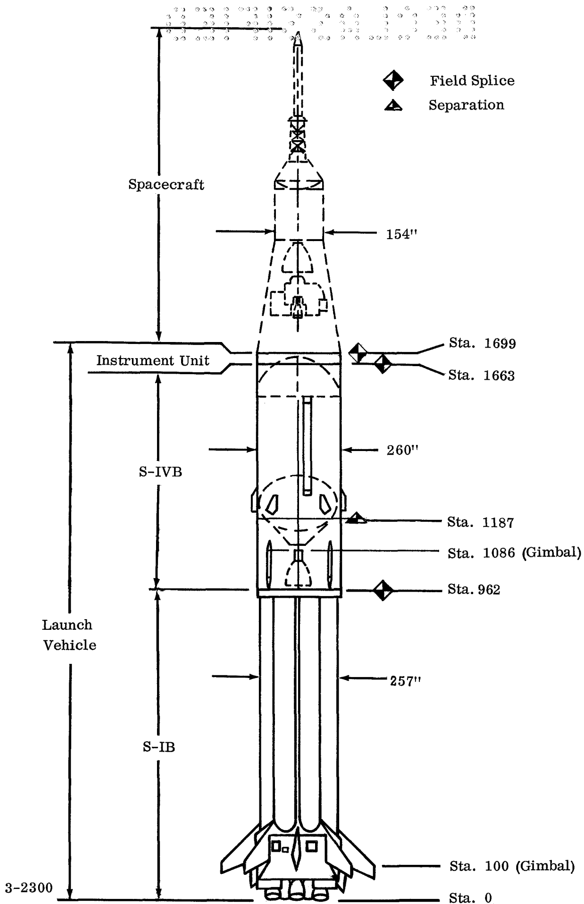
Figure 12-1. Saturn IB Launch Vehicle
