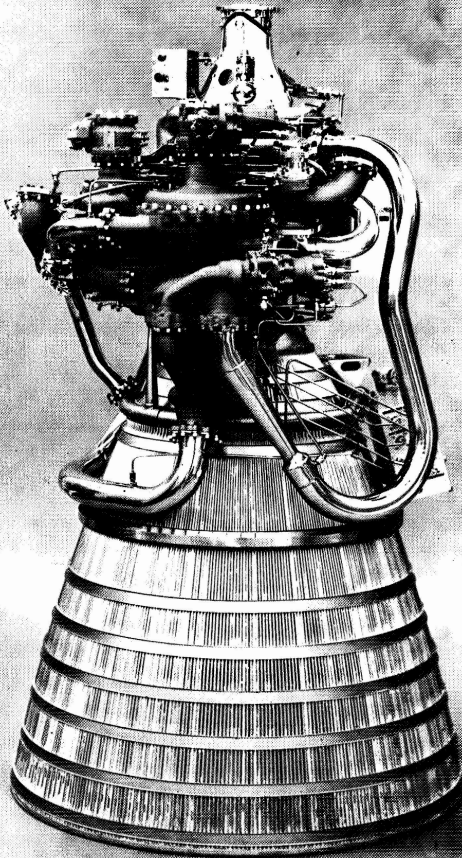
Figure 8-13. RL10A-3 Engine
