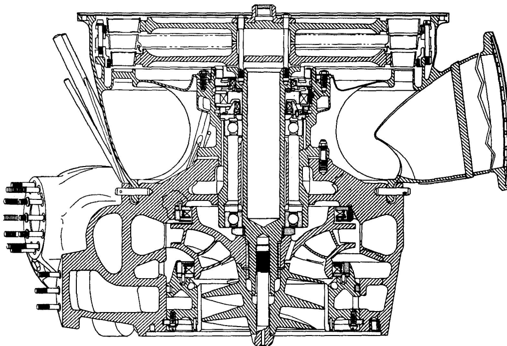
Figure 22-13. J-2 Oxidizer Turbopump
