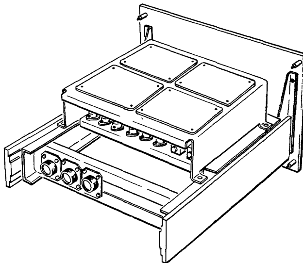
Remote Propellant Loading Relay Assembly
