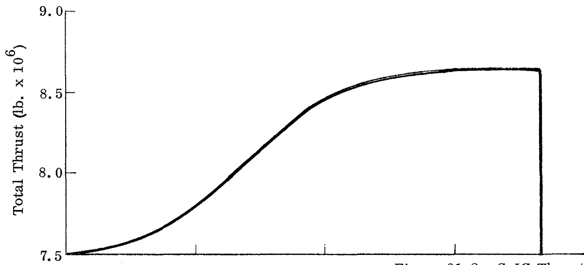
Figure 21-2. S-IC Thrust
