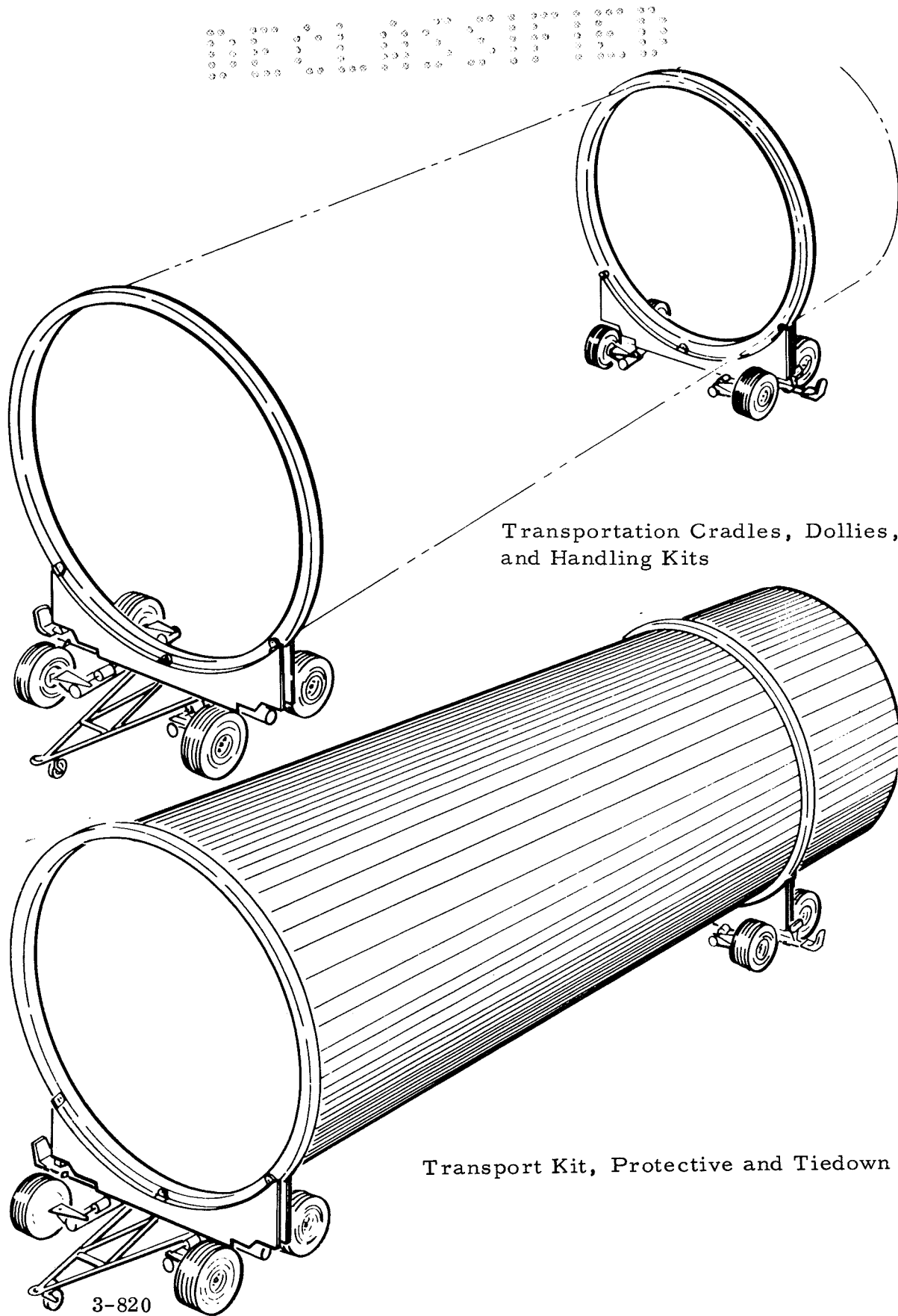
Figure 17-2. Transportation, Protection, and Handling Equipment,S-IVB (1 of 4)
