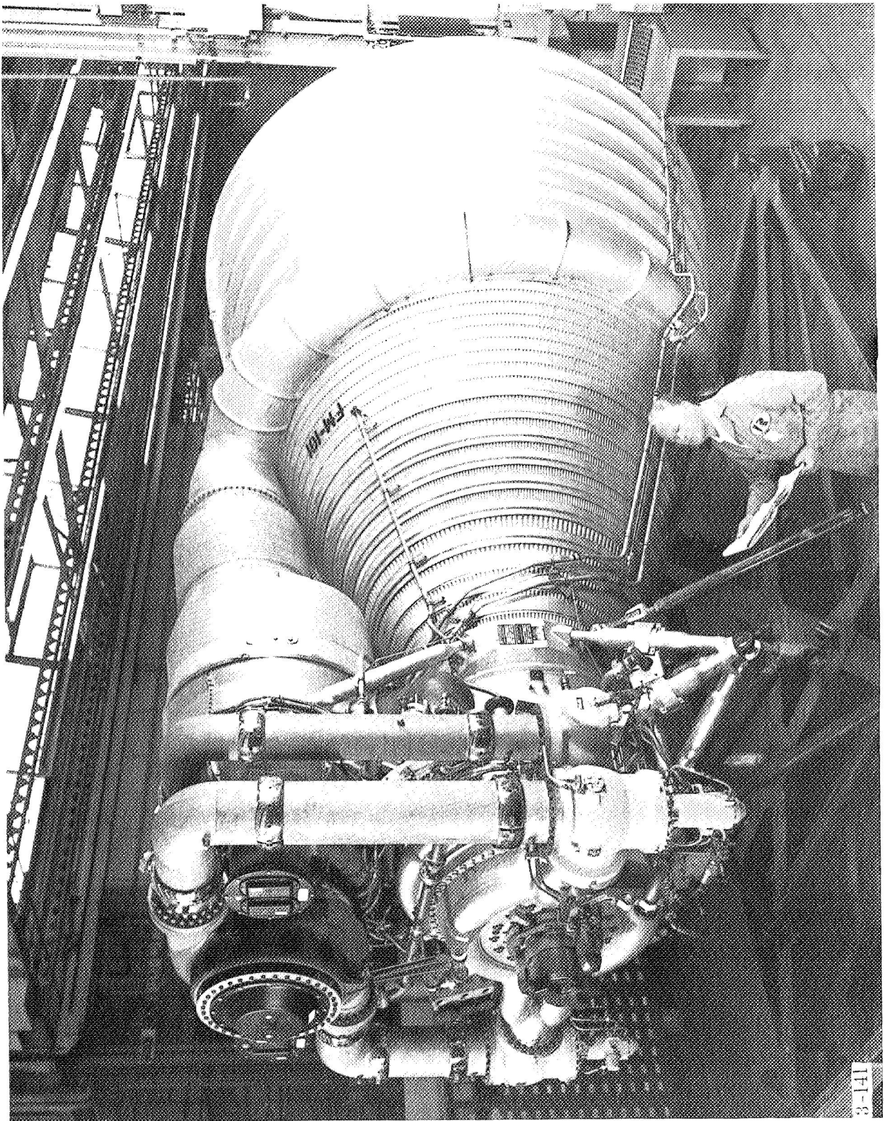
Figure 22-3. F-1 Engine
