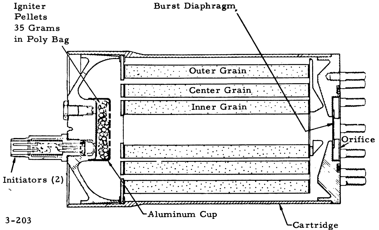
Figure 9-10. Solid-Propellant Gas Generator
