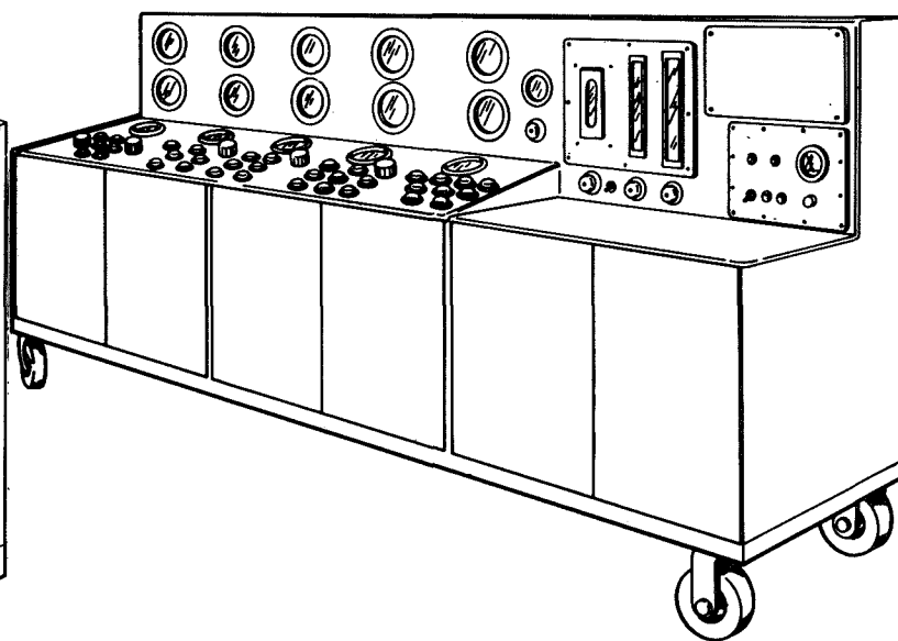
Stage Checkout Area Pneumatic Console - Checkout Accessories
