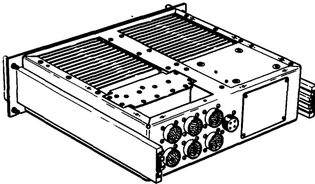
Flight Sequence Recorder Chassis
