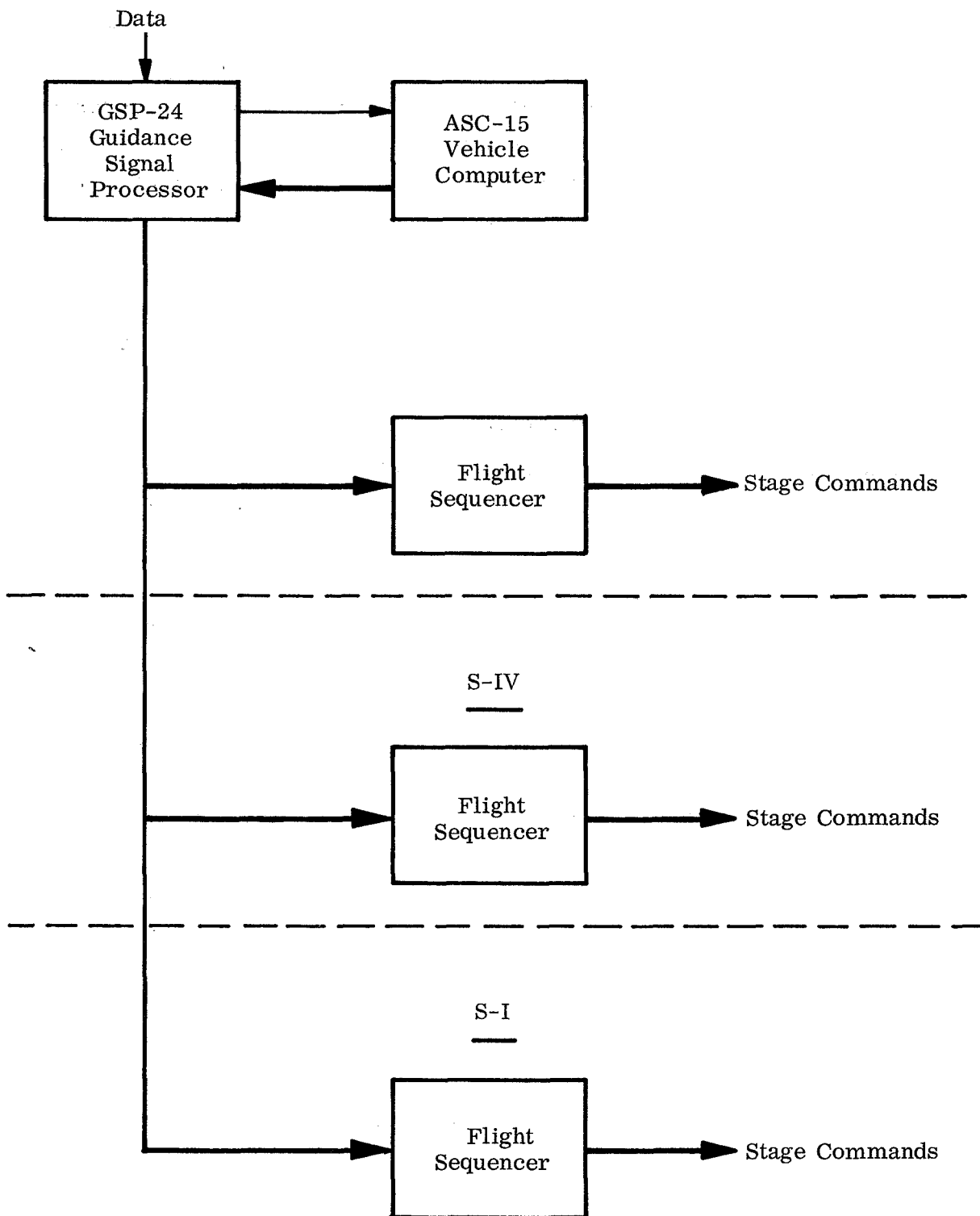
Figure 6-2. Ascent Phase Command Configuration, Saturn I
