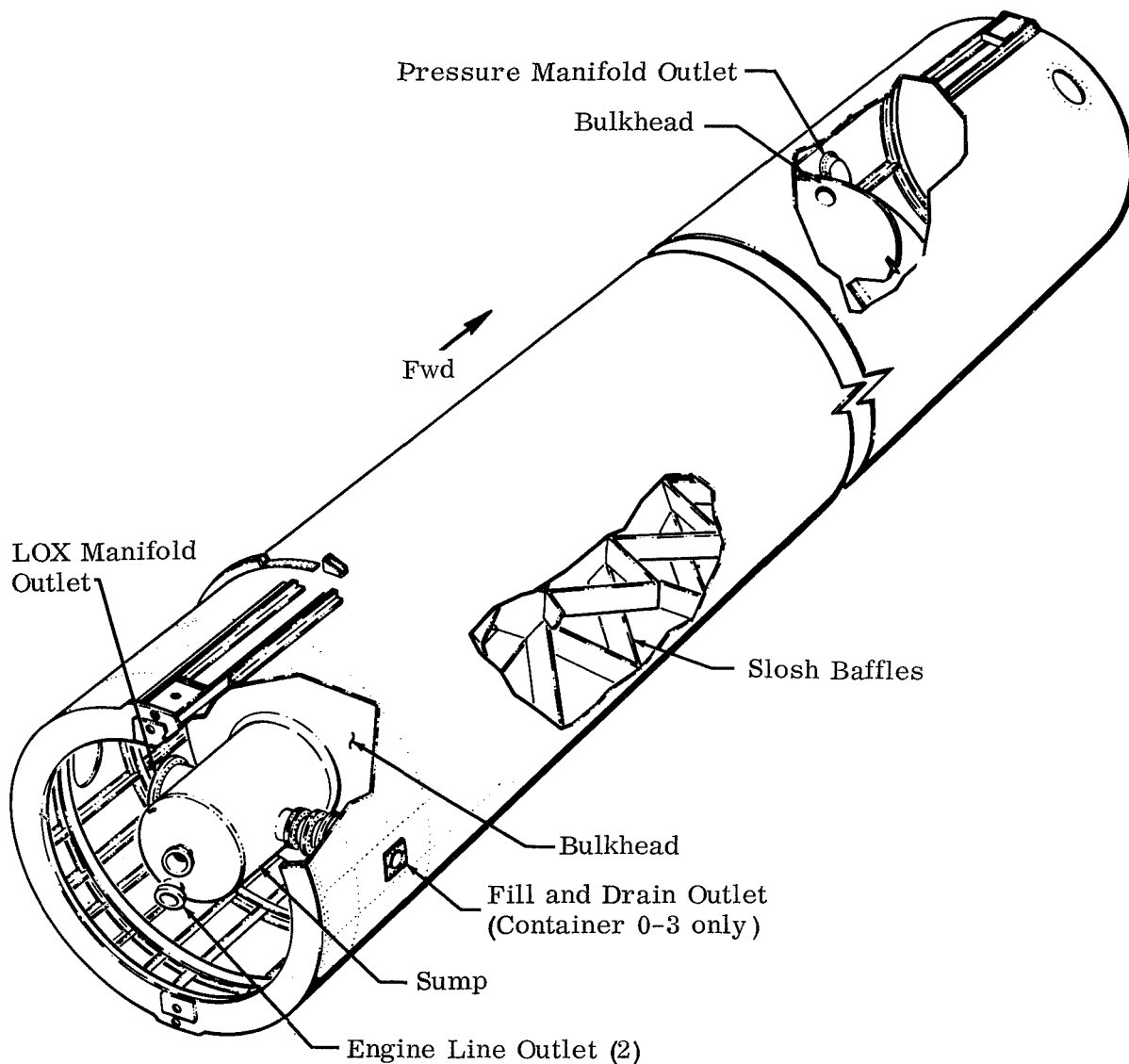
Figure 7-8. Outboard LOX Container (0-3), S-I
