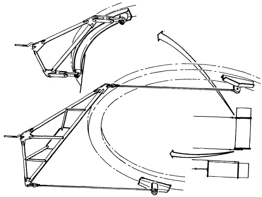
Hoist Kit
