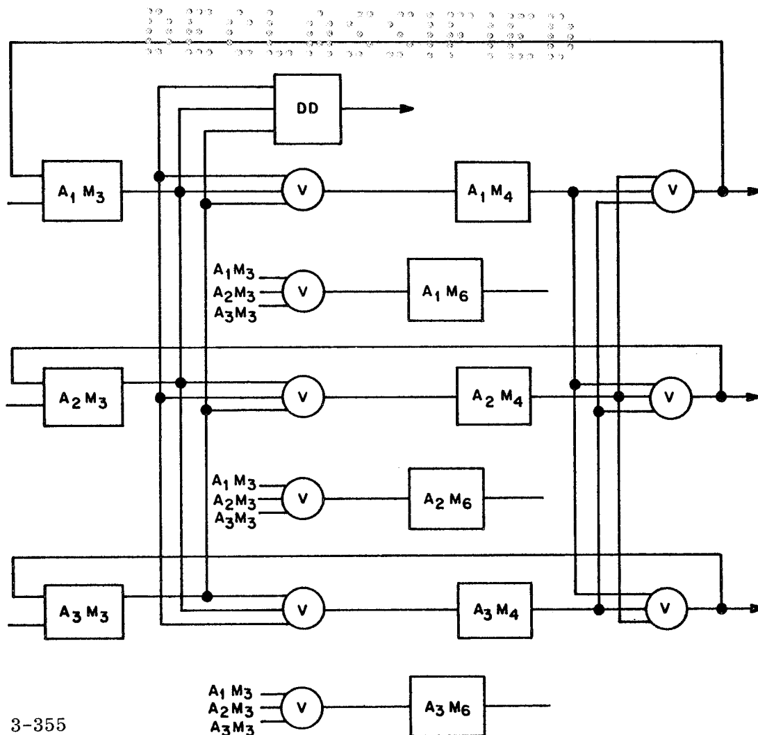
Figure 20-27. Triple Modular Redundancy Voter Signal Outputs
