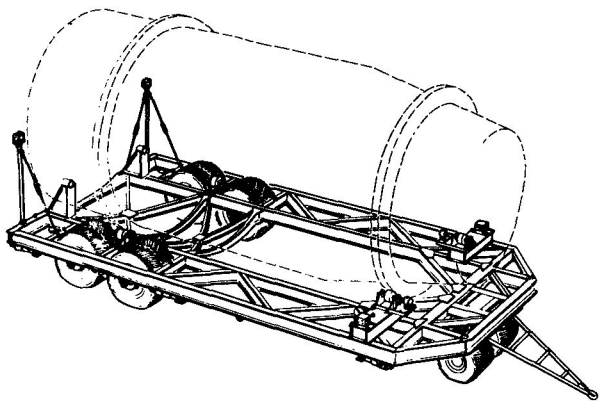
Transporter Assembly
