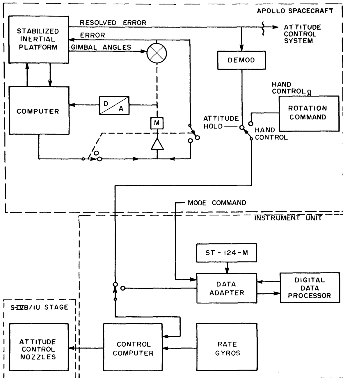
Figure 20-18. Rotational Command Control Mode
