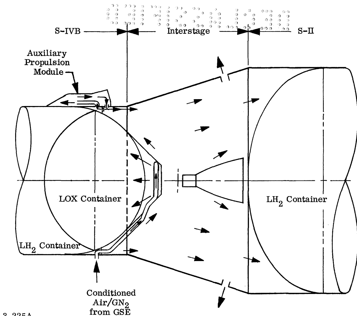
Figure 23-4. Interstage Compartment Environmental Control, S-II/S-IVB
