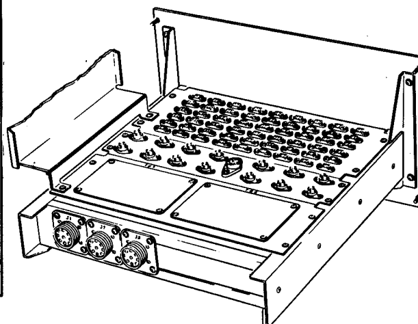
Flight Sequence Control Chassis Nos. 1 and 2 (Typical)
