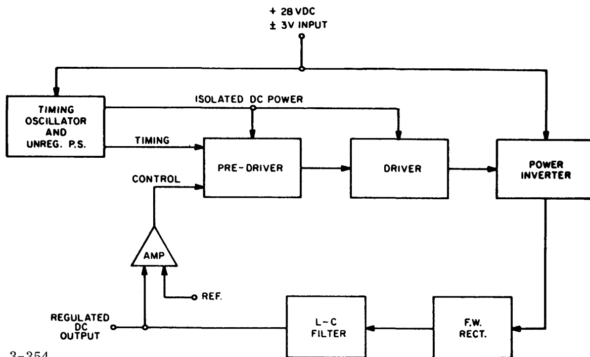
Figure 20-26. Pulse-Width-Modulated Power Supply Module Block Diagram
