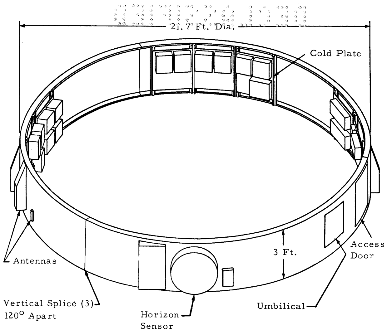
Figure 21-14. Instrument Unit, Saturn V
