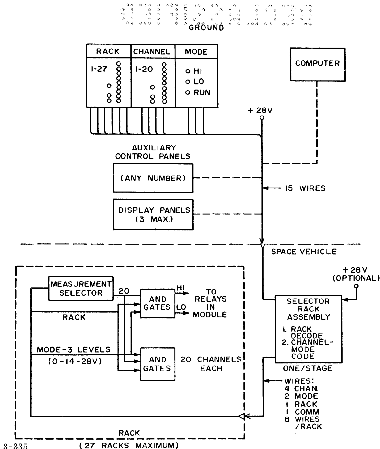
Figure 20-7. Remote Automatic Calibration System (RACS) Block Diagram
