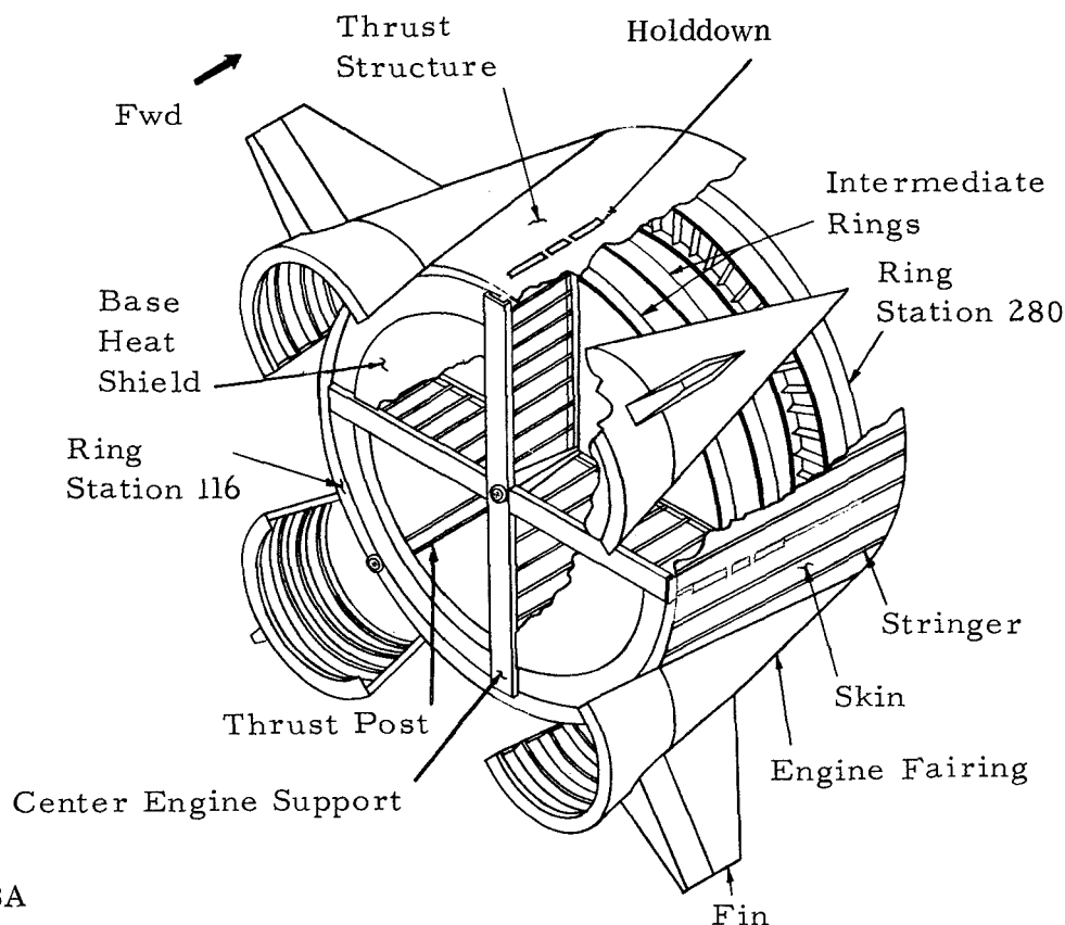
Figure 21-5. Thrust Structure, Fins, Engine Fairings, S-IC
