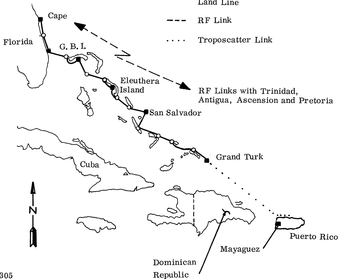
Figure 6-3. AMR Submarine Cable
