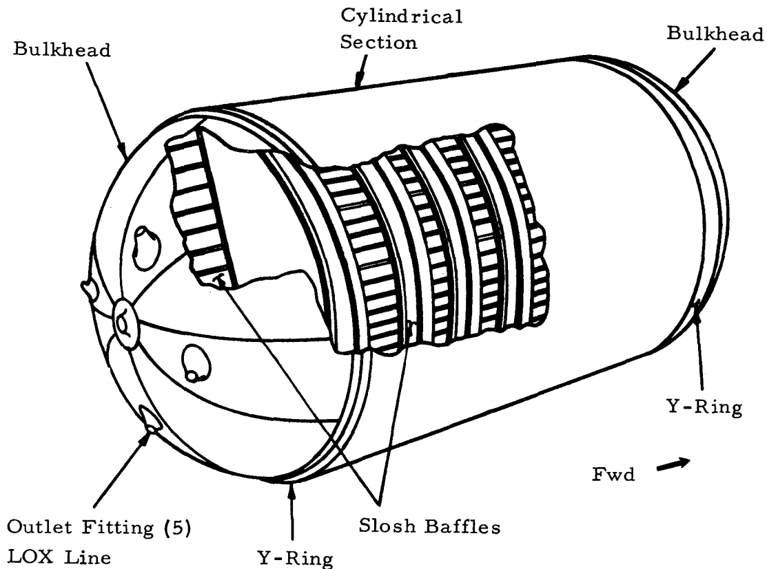
Figure 21-10. Oxidizer Container, S-IC
