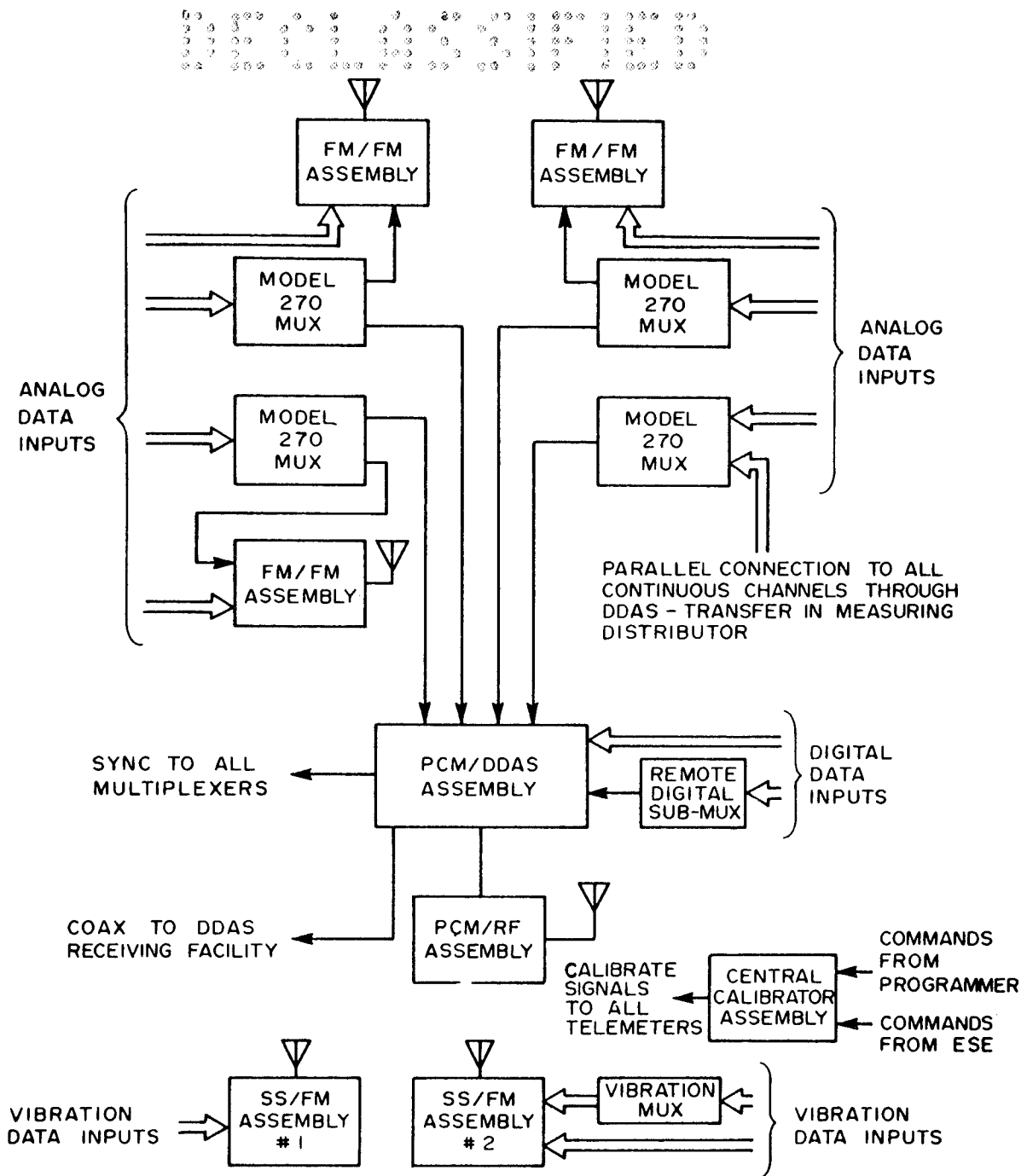
Figure 20-9. Typical Stage Telemetry System, Saturn V
