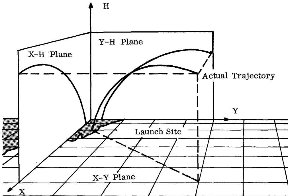
Figure 6-27. Three Coordinate Projection of Saturn Trajectory
