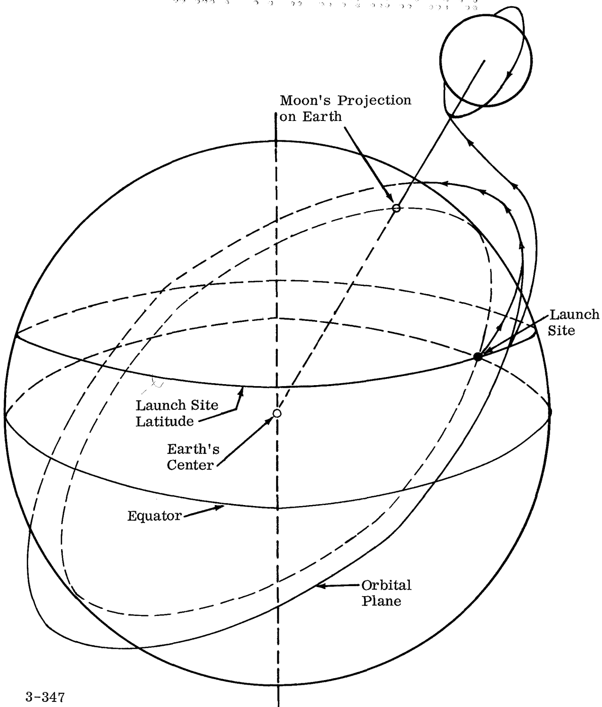
Figure 20-19. Variable-Inclination Earth-Orbital Plane
