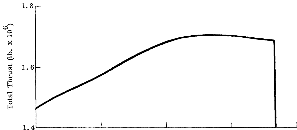
Figure 7-2. S-I Thrust
