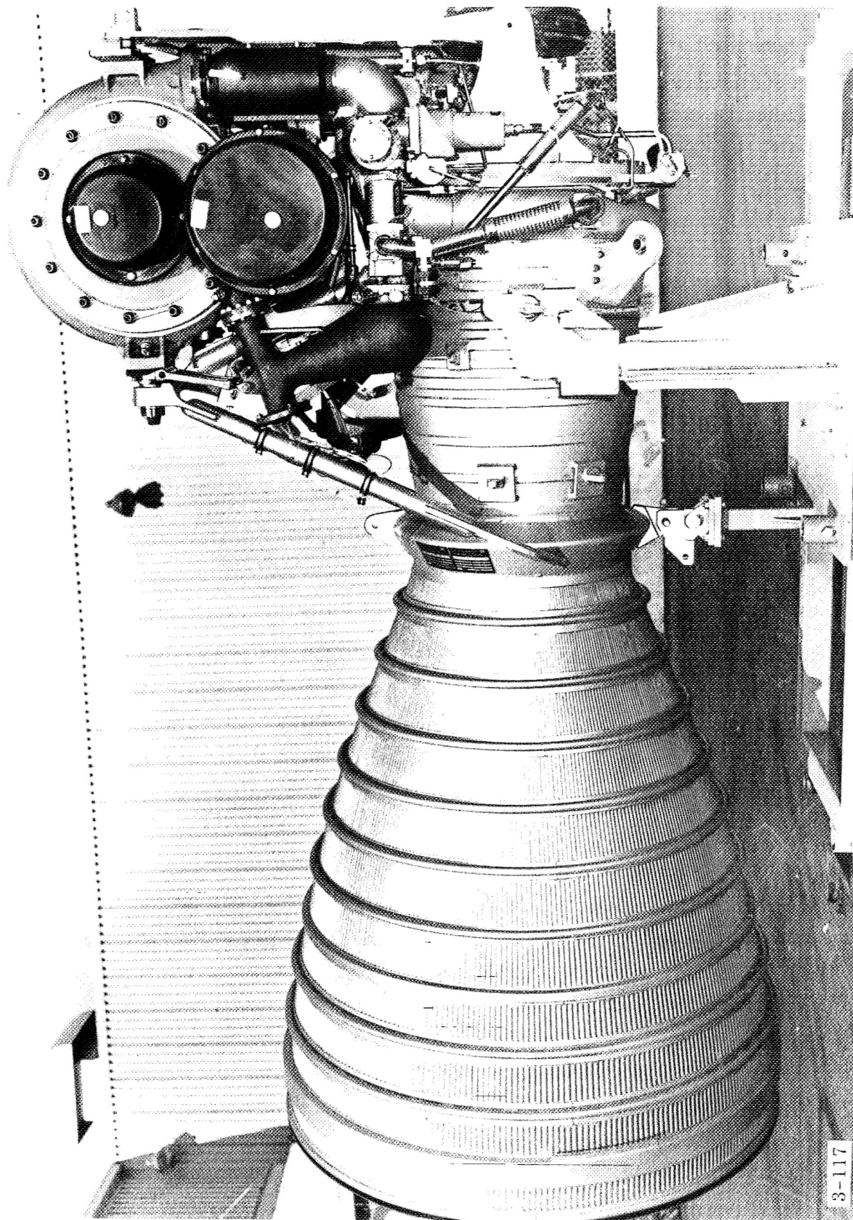
Figure 8-3. H-1 Engine
