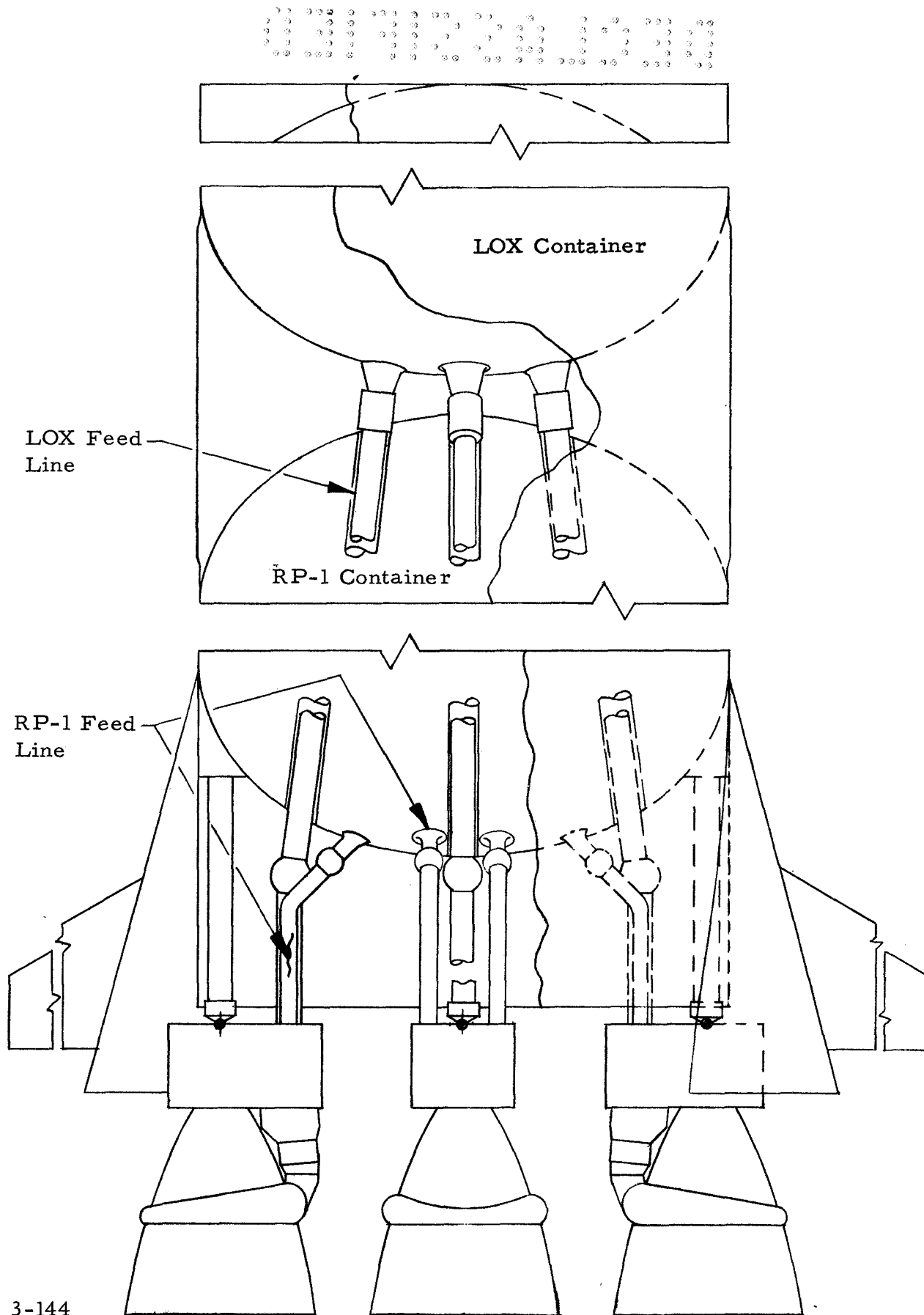
Figure 22-7. Propellant System, S-IC
