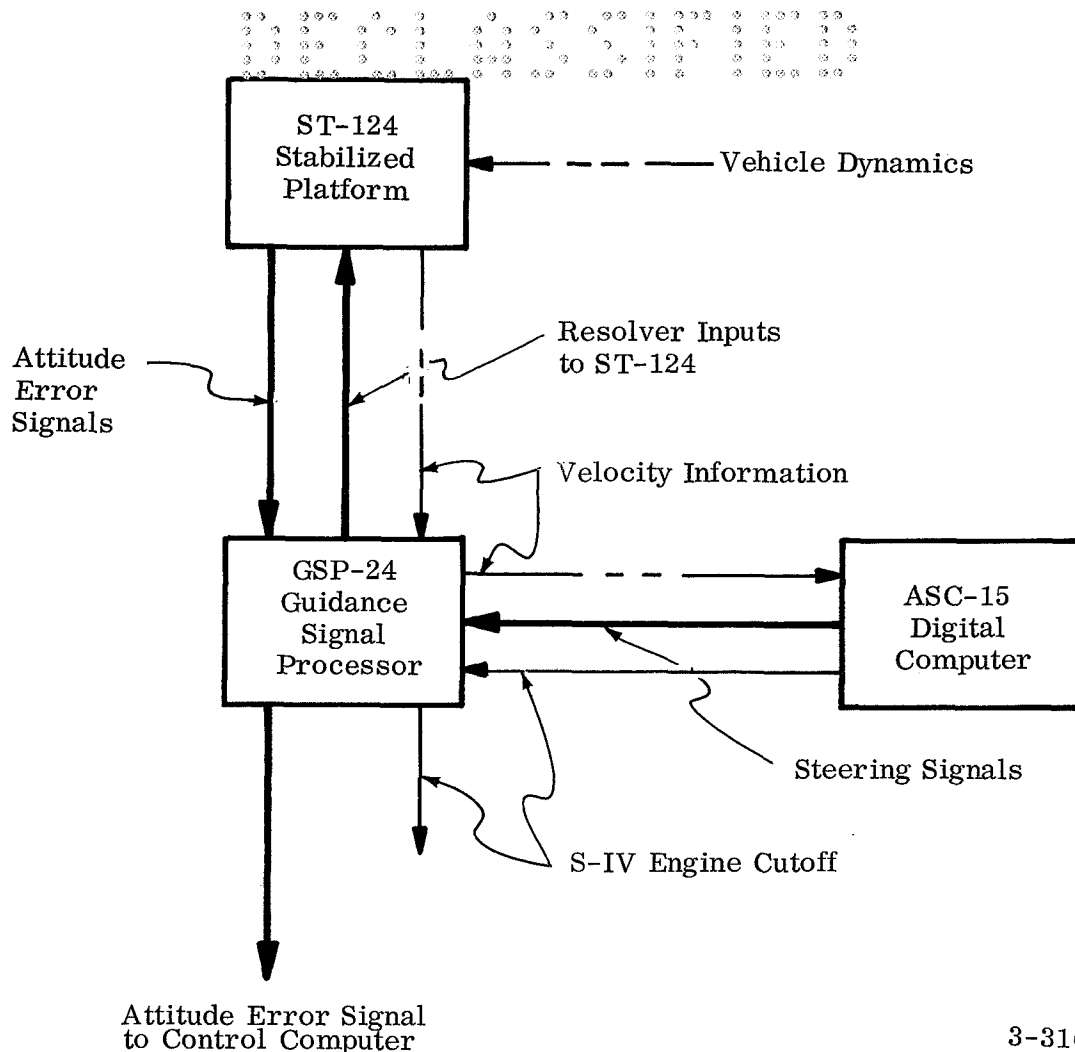
Figure 6-19. Guidance Implementation, Saturn I
