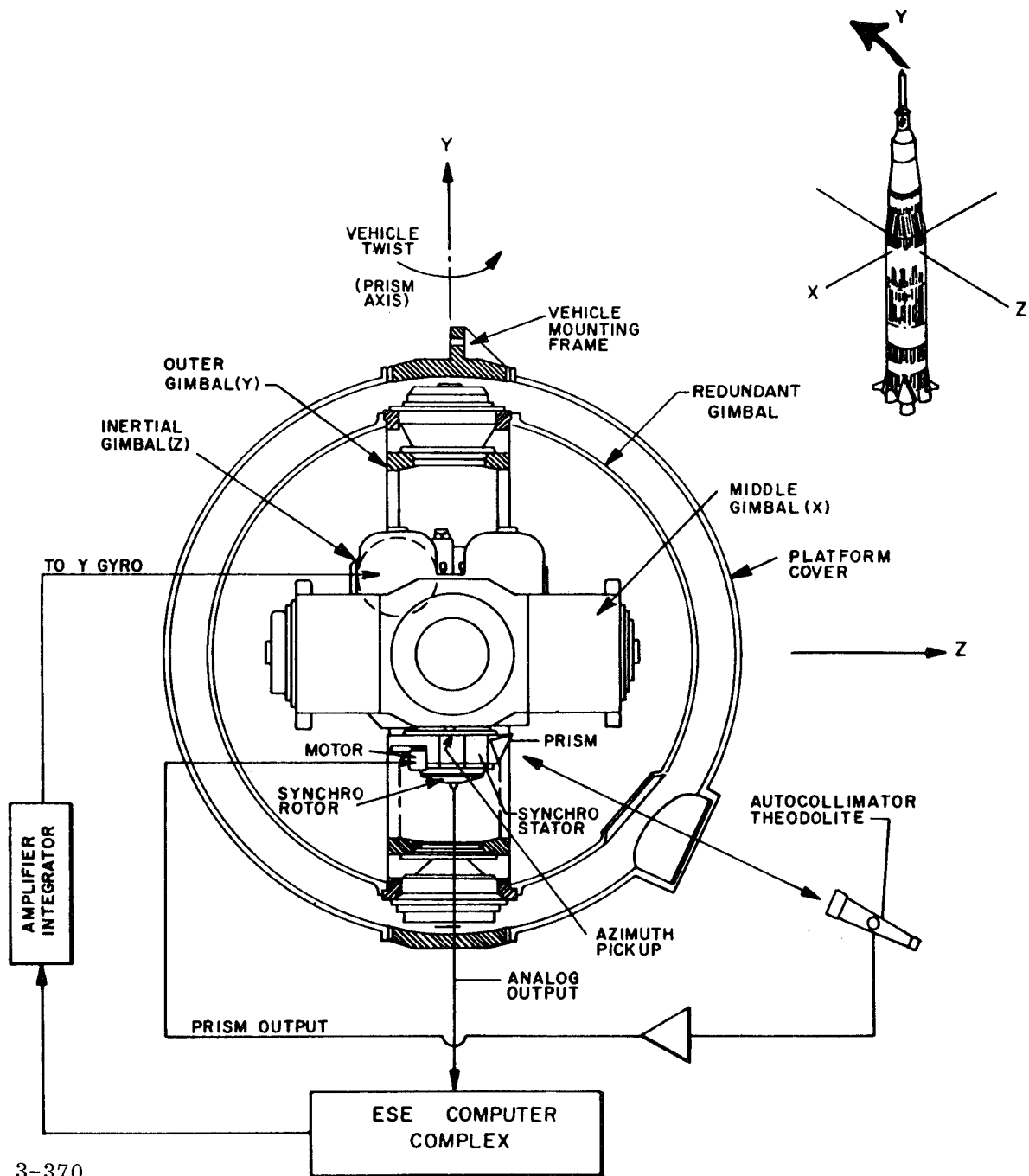
Figure 20-41. Automatic Azimuth Alignment
