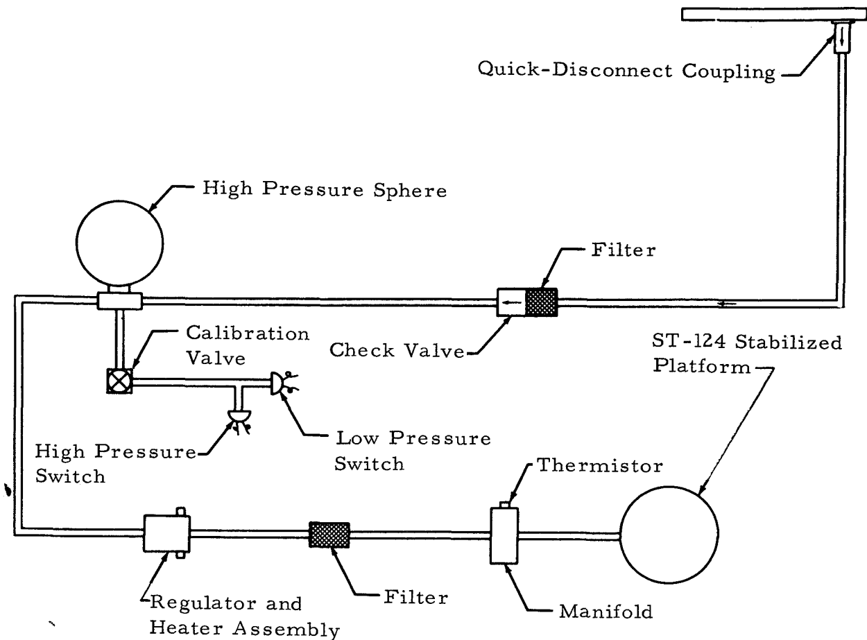
Figure 9-23. Platform Gas-Bearing Supply System
