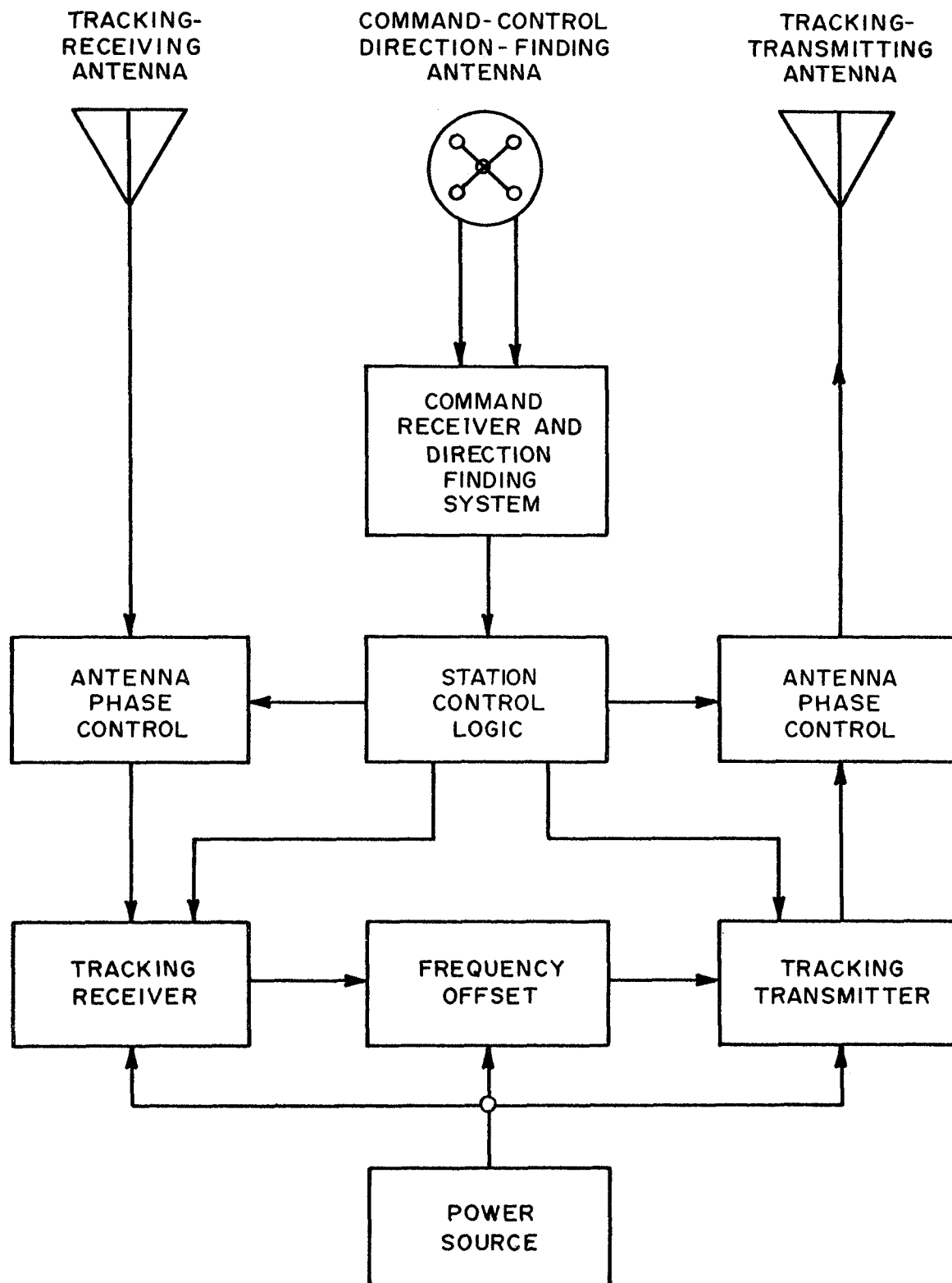
Figure 13-2. AROD Transponder Ground Station
